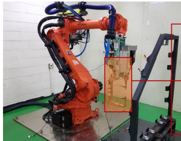
Experiment Testbed
