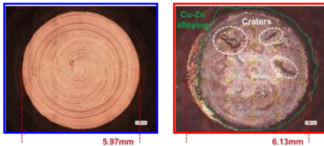
Welding electrode tip (Normal / Abnormal)
